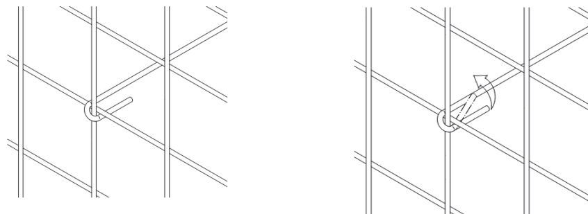
Figure: Correctly bended stay rods
