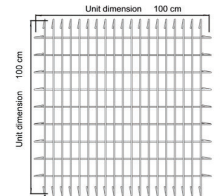
Figure: monotec ® grill
